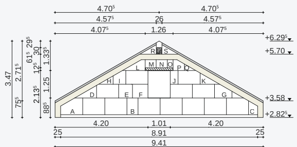
Giebelwand
