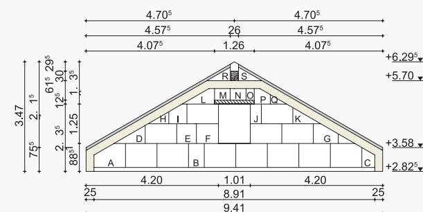
Giebelwand
